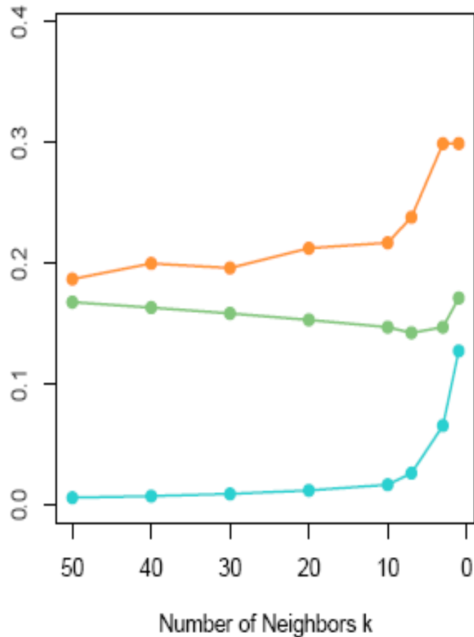
k-NN - Classification
