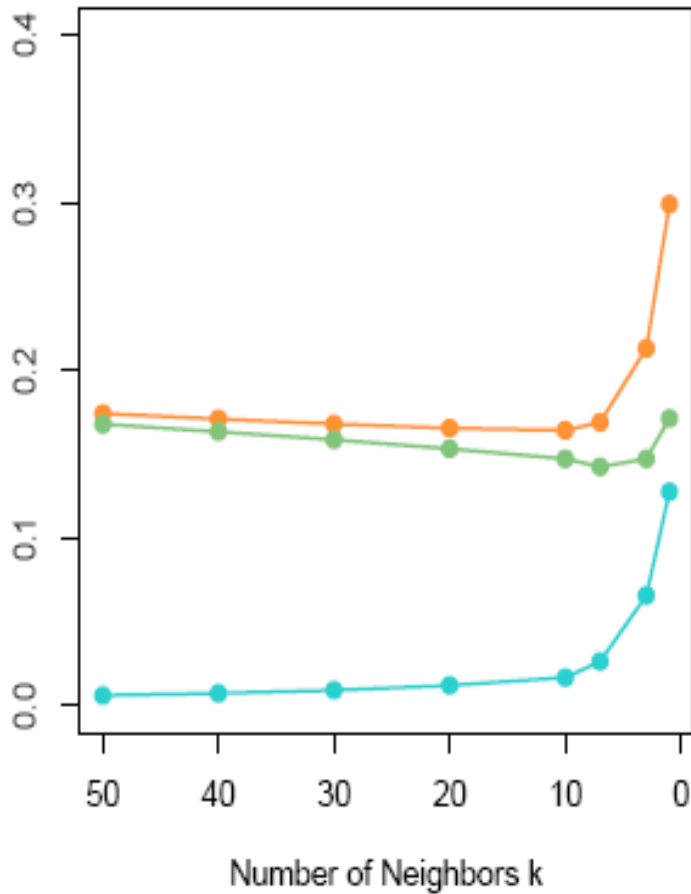
k-NN - Regression
