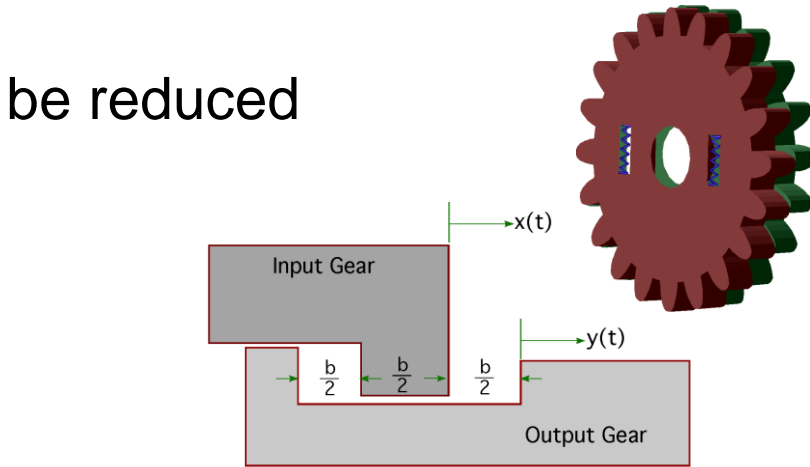
Input Gear Tooth Shown Centered Between Two Output Gear Teeth
